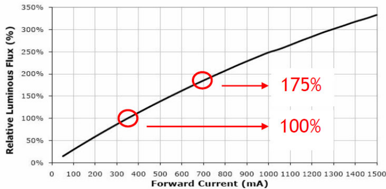
Relative Flux vs. Current ( T_j = 25^\circ\text{C} )
